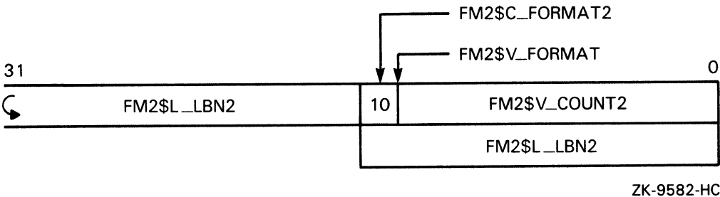
Figure 2-7: Retrieval Pointer Format 2
