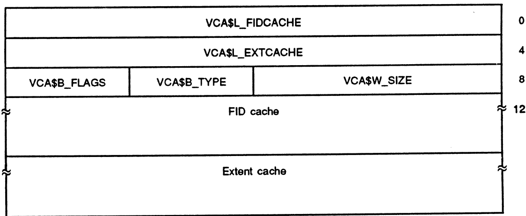
Figure 4–15: Format of the Volume Cache Block
